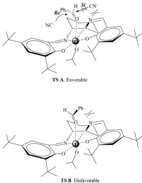
Figure 3. The potential transition states.
