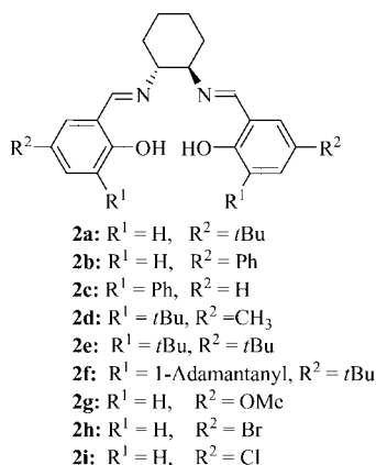
Figure 2. Ligands assessed in this study.
