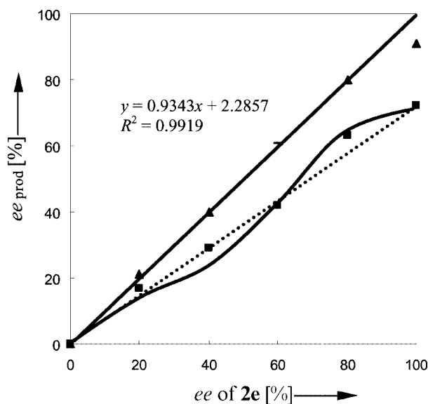
Figure 1. Studies of the nonlinear effect in the reaction between benzaldehyde and ethyl cyanoformate in an i PrOH/CHCl 3 mixture (1:4 v/v, 0.8 mL) as solvent (▲), and in chloroform as solvent (■).
